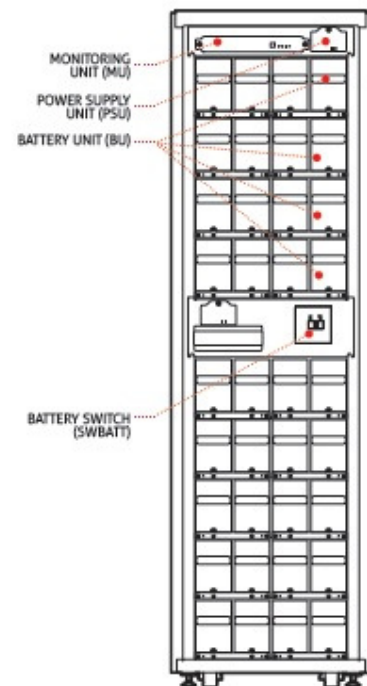
MPW Battery Cabinet (front)
