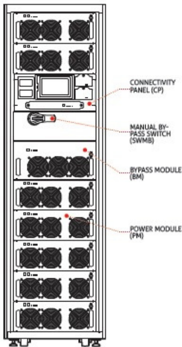
MPW Power Cabinet 42-294 kW (front)
